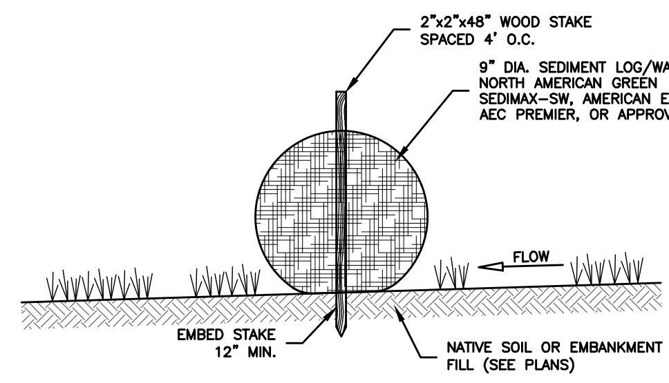
STORMWATER SEDIMENT LOG (WATTLE) DETAIL NOT TO SCALE
