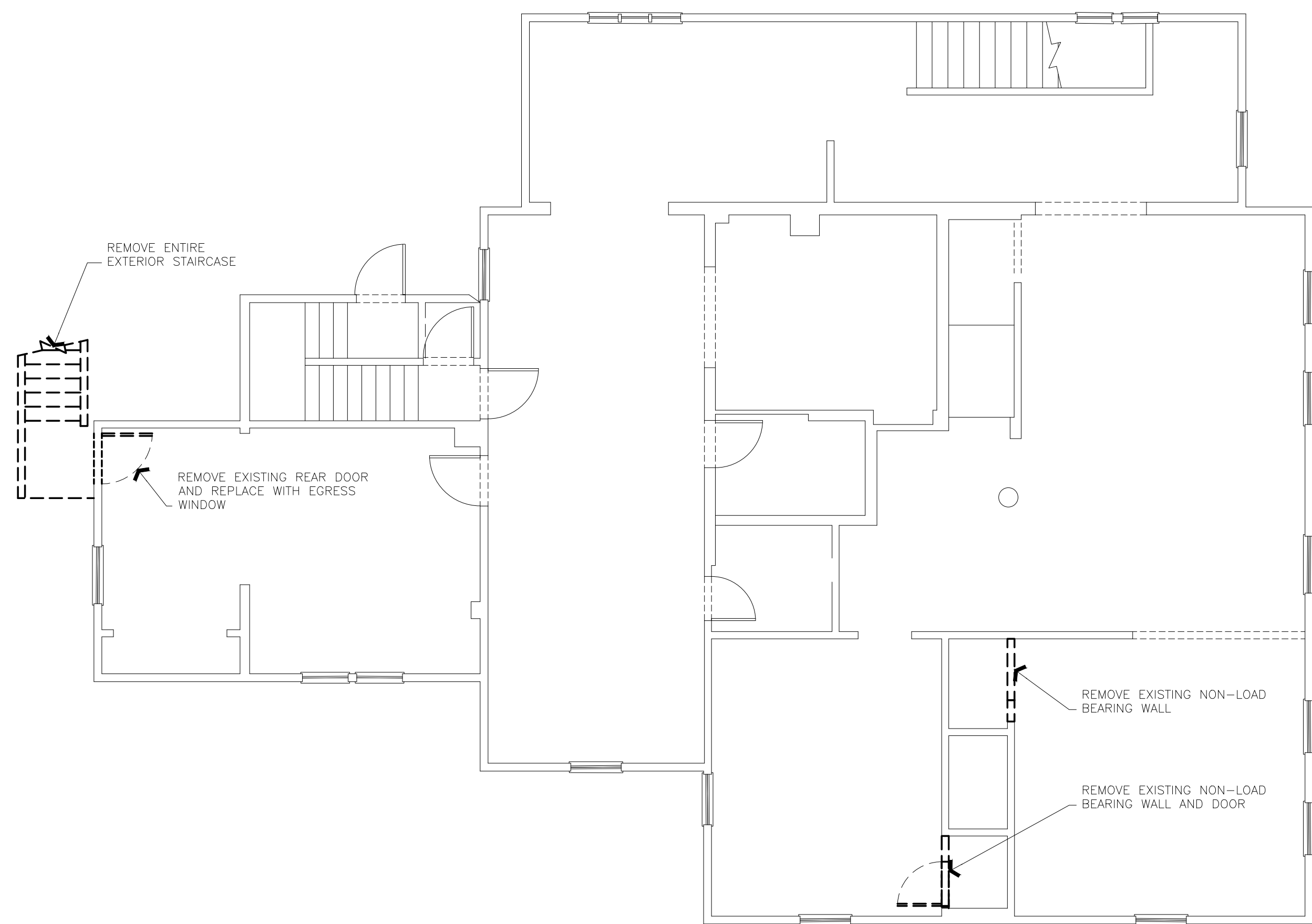
1 UPPER FLOOR ALTERATION PLAN A1.2 SCALE: 3/16"=1'-0"
