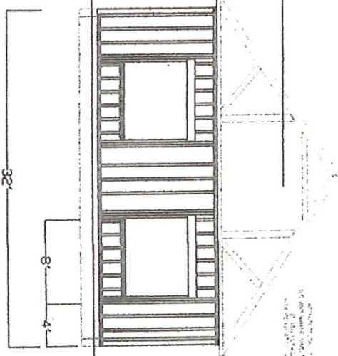
ELEVATION LOOKING EAST - POOL BUILDING
